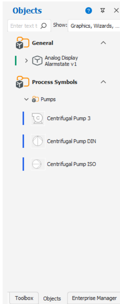
Figure 1: Objects Toolbox
